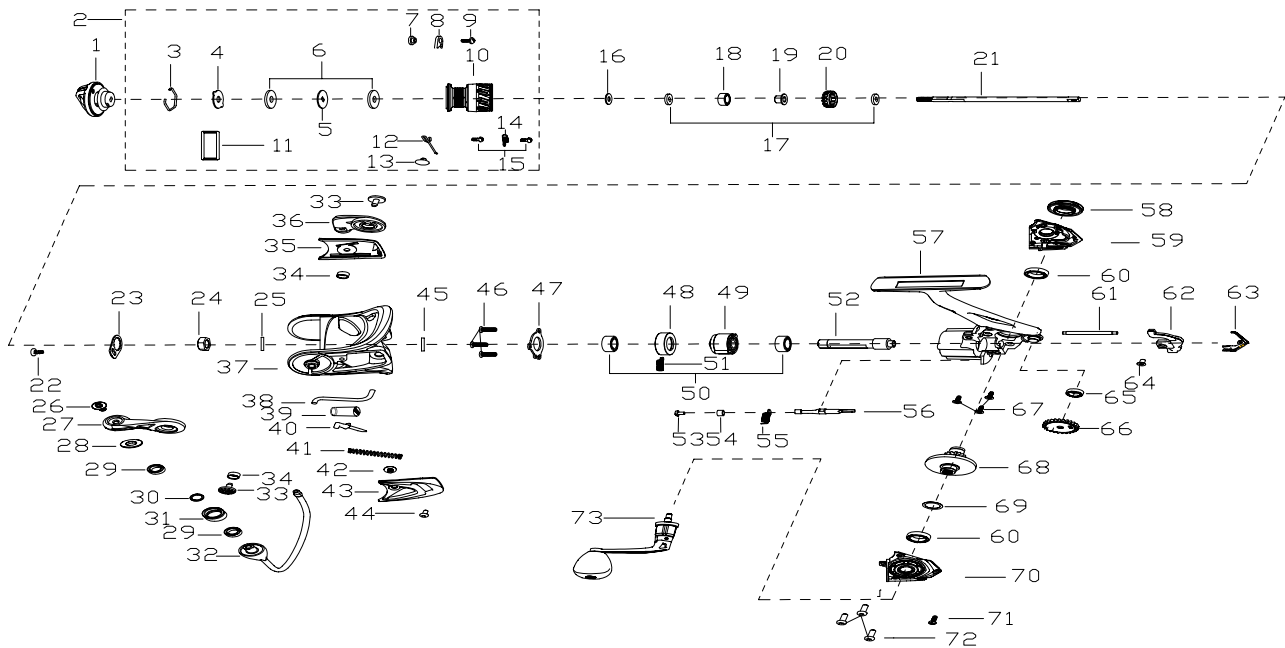
PARTS LIST OF CS6-1000
