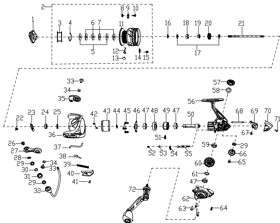
EXPLODED VIEW OF CS10-2000
